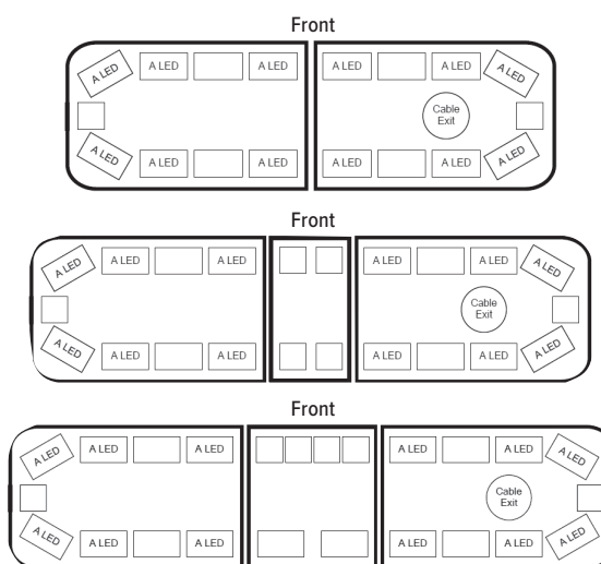
Pre-Configured Lightbars
